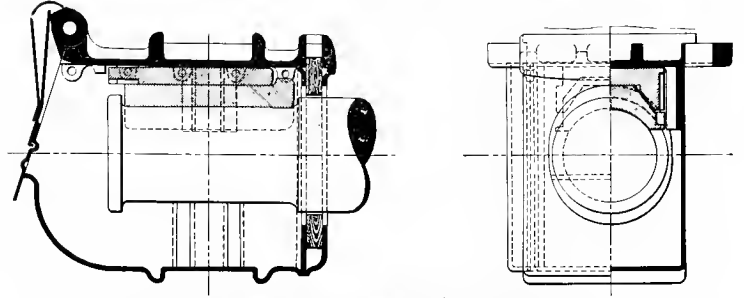
Figs. 5163-5164. Longitudinal and Cross Sections. SCHOEN SOLID PRESSED-STEEL JOURNAL-BOX.
